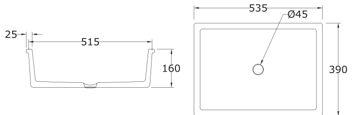
Wash Basin (Table Top)
